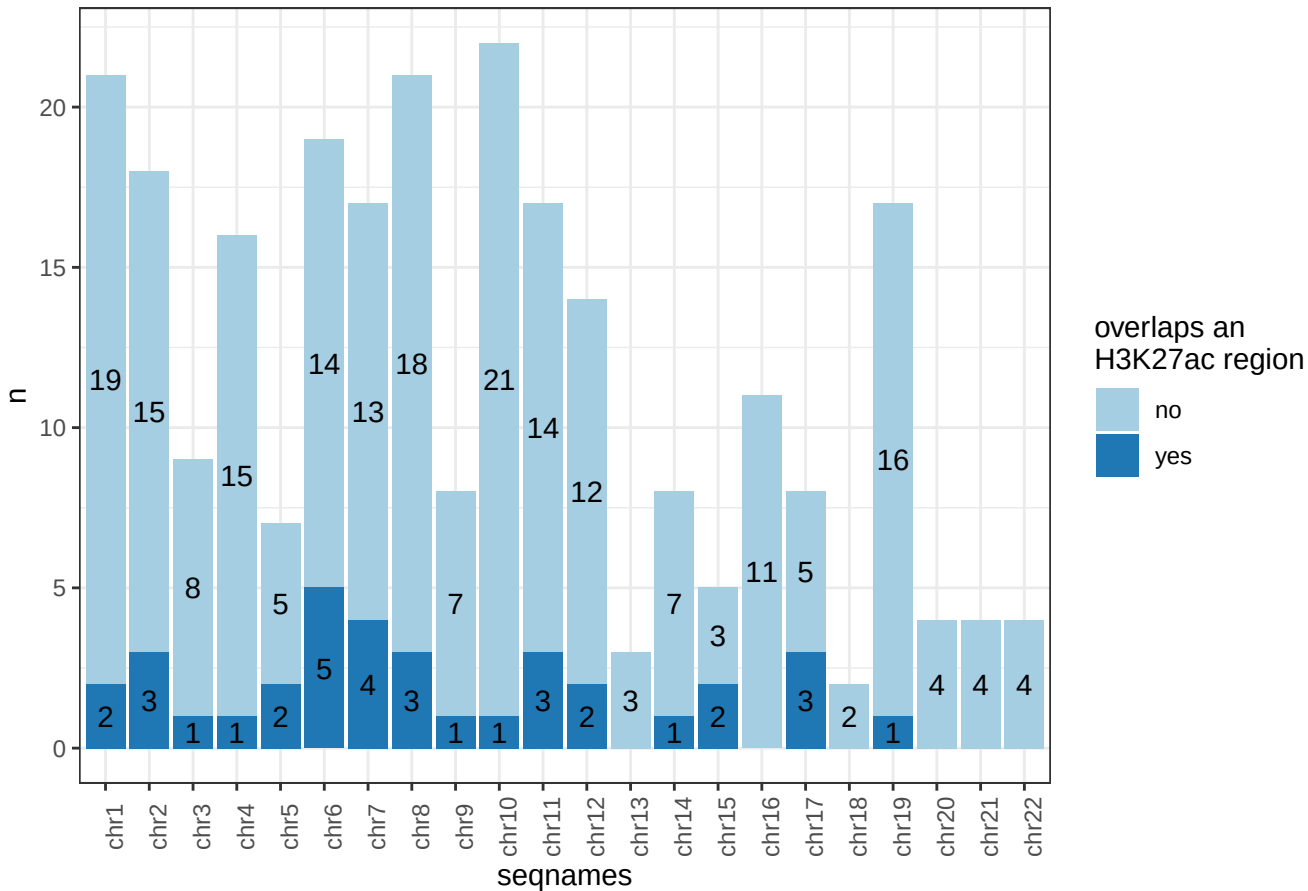
LTR10E distribution across chromosomes
